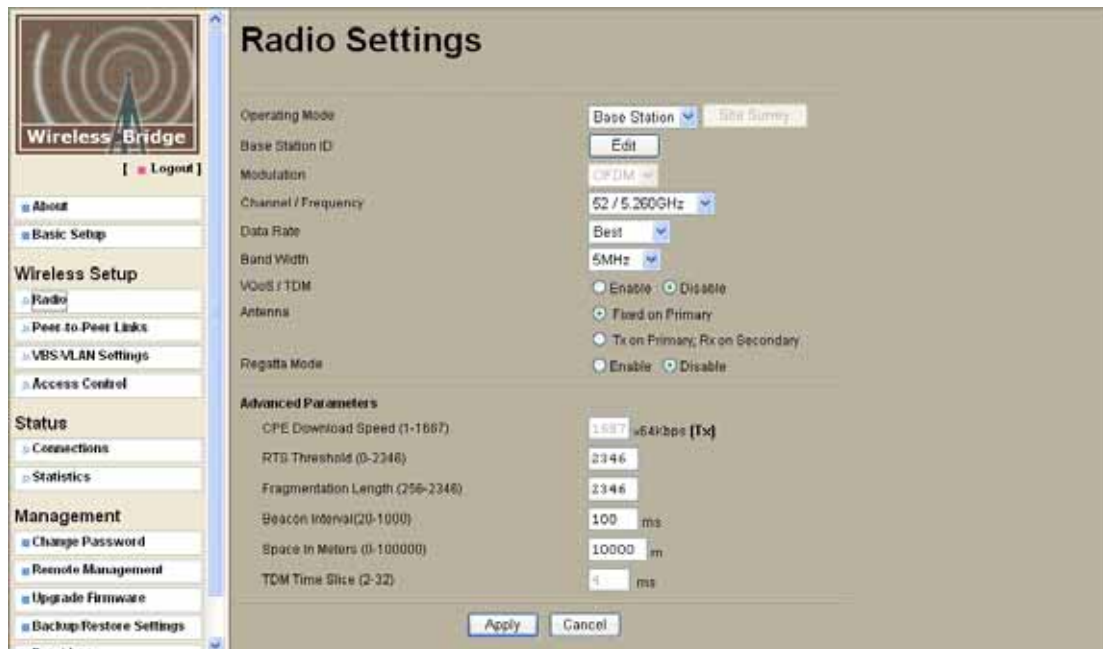
Figure 7 Base Station Mode
