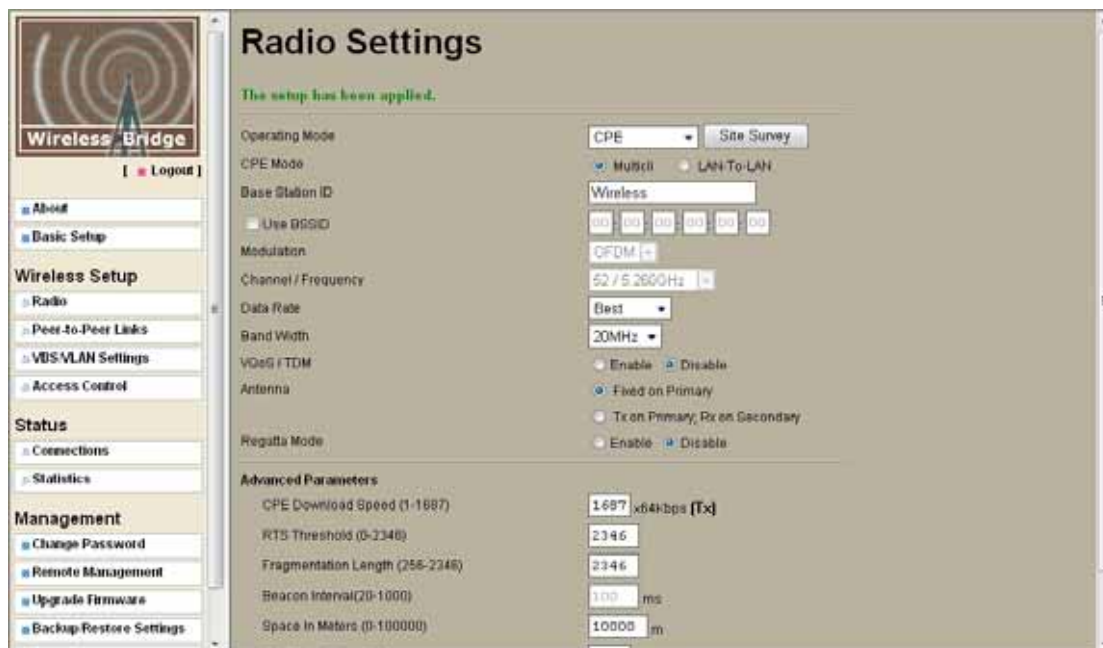
Figure 8 CPE Mode
